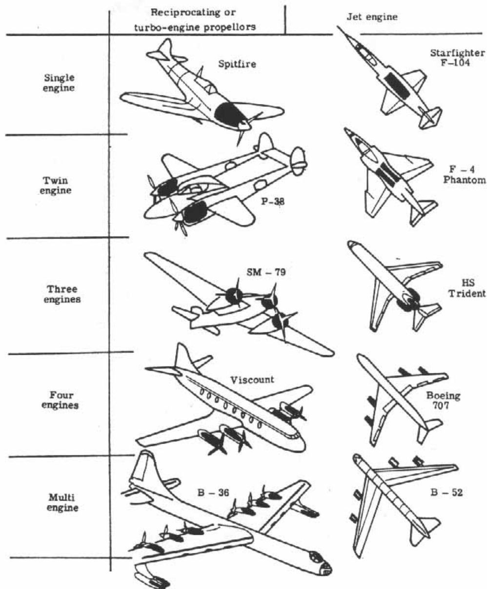
Figure 18.- Power-plant placement.
