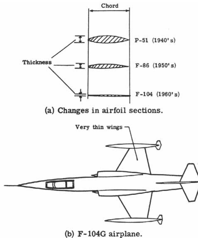
Figure 89.- Thin airfoils.
