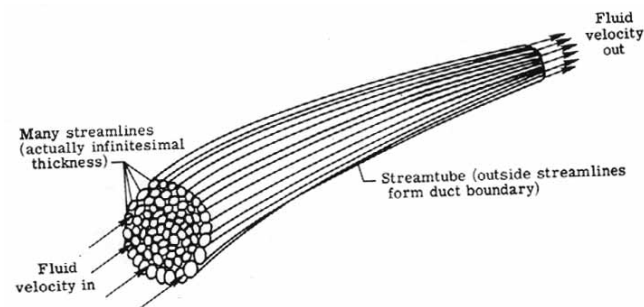
(a) Stream tubes.
