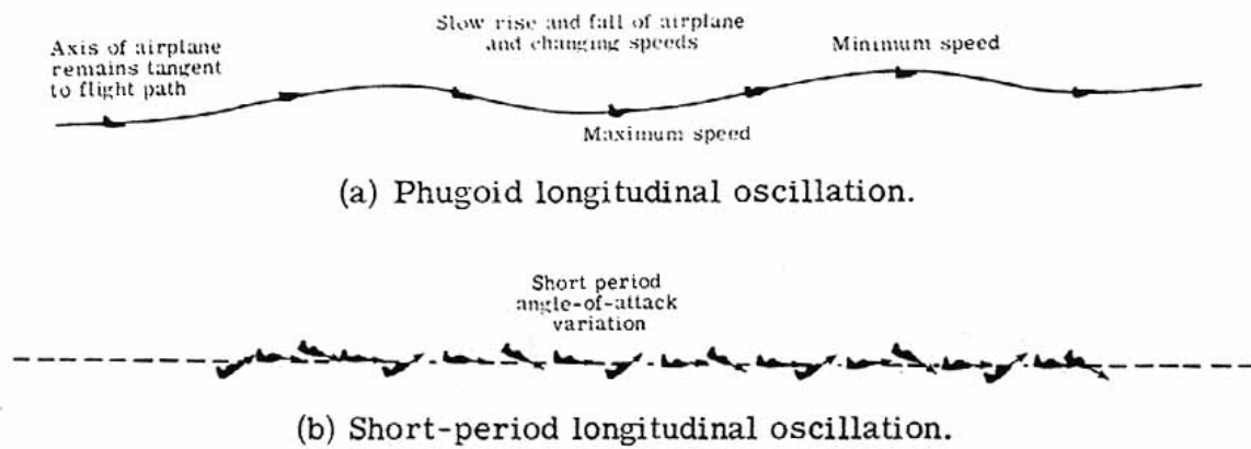
Figure 137.- Two types of dynamic longitudinal oscillations.
