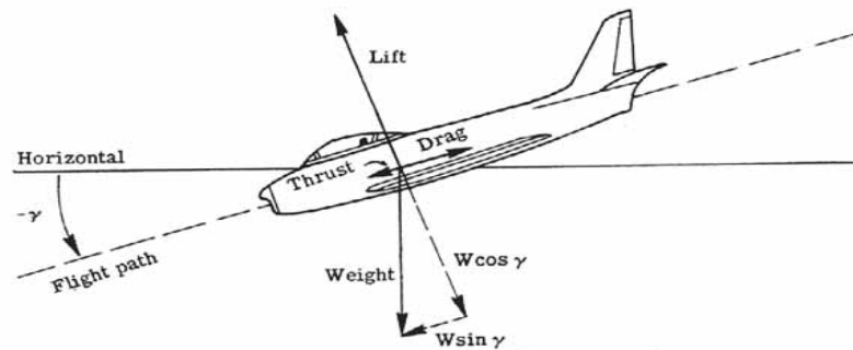
(b) Dive, unaccelerated.
