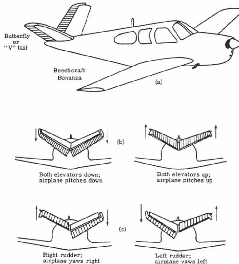
Figure 159.- Butterfly tail operation.
