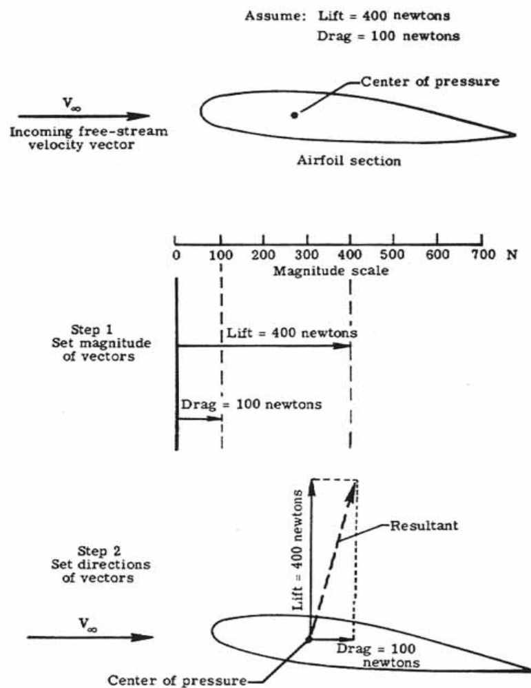
Figure 161.- Vector representation.
