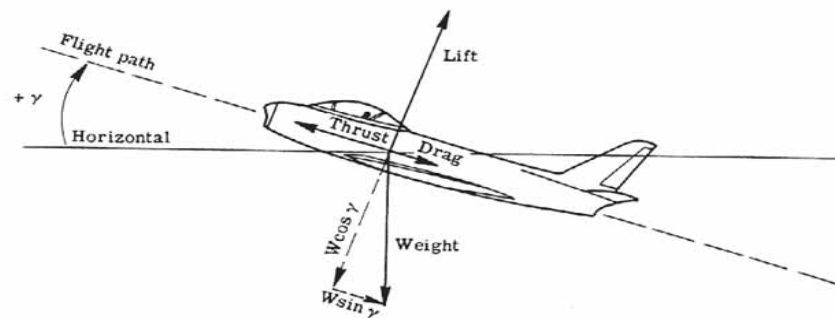
(a) Climb, unaccelerated.
