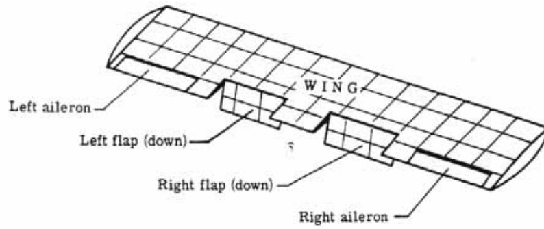
(a) Simple flap arrangement.
