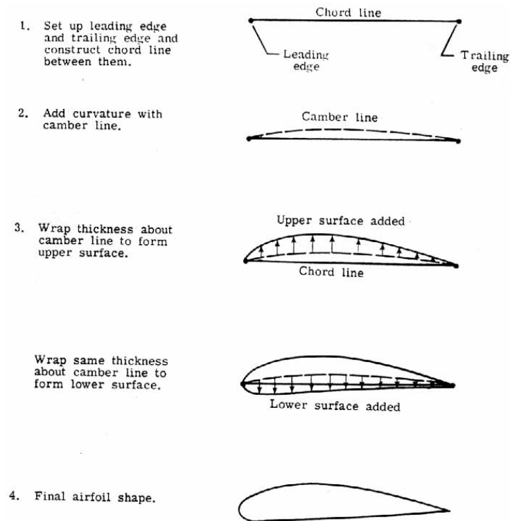
Figure 40.- Geometric construction of an airfoil.
