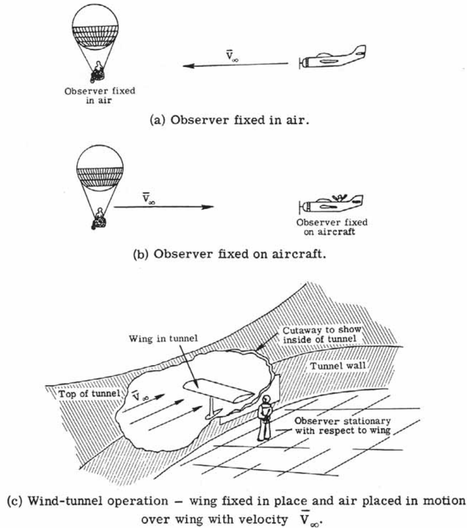
Figure 162.- Relative motion.
