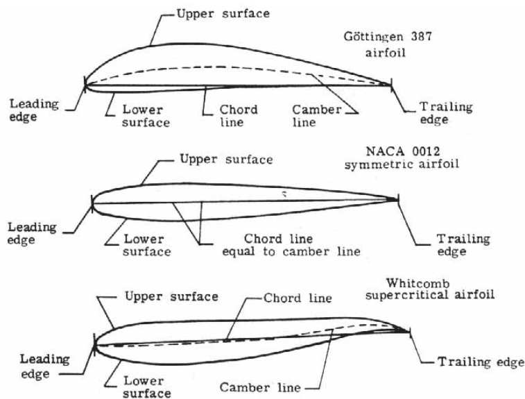
Figure 41.- Airfoil terminology.
