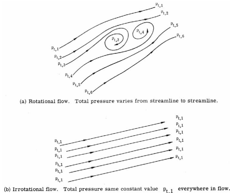
Figure 26.- Total-pressure variation.
