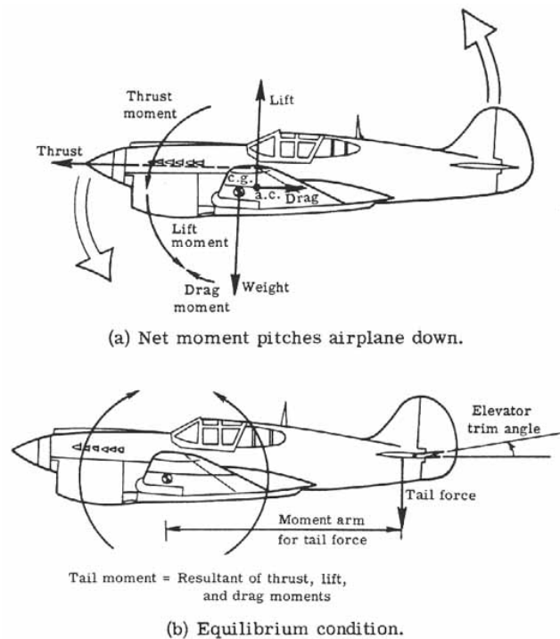
Figure 131.- Pitch equilibrium.
