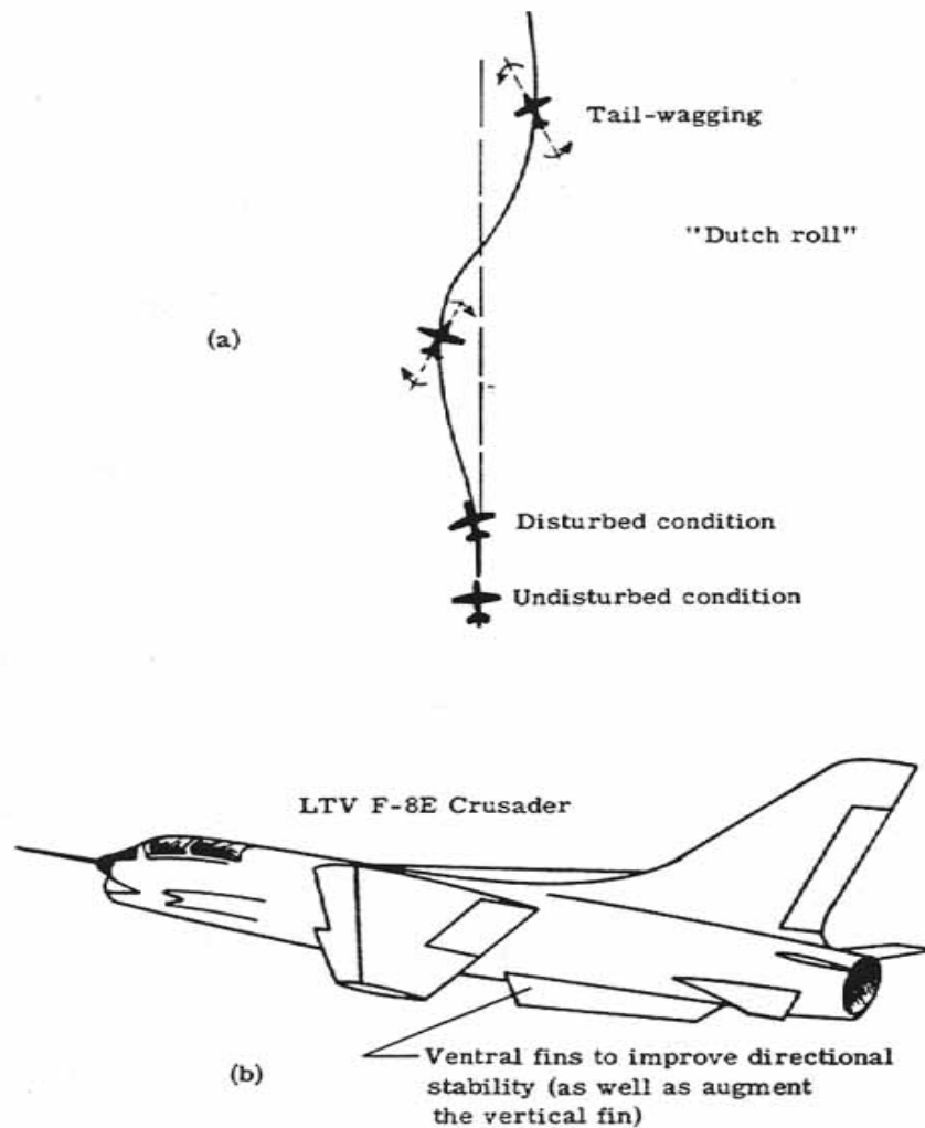
Figure 149.- Dutch roll.
